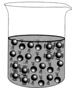
(b) Liquids: particles are free to move within the liquid. Some particles escape the surface to form a vapour.
