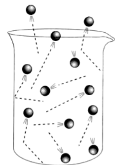
(c) Gases: particles move freely in all directions. Gases are compressible since there is a lot of space between particles.
